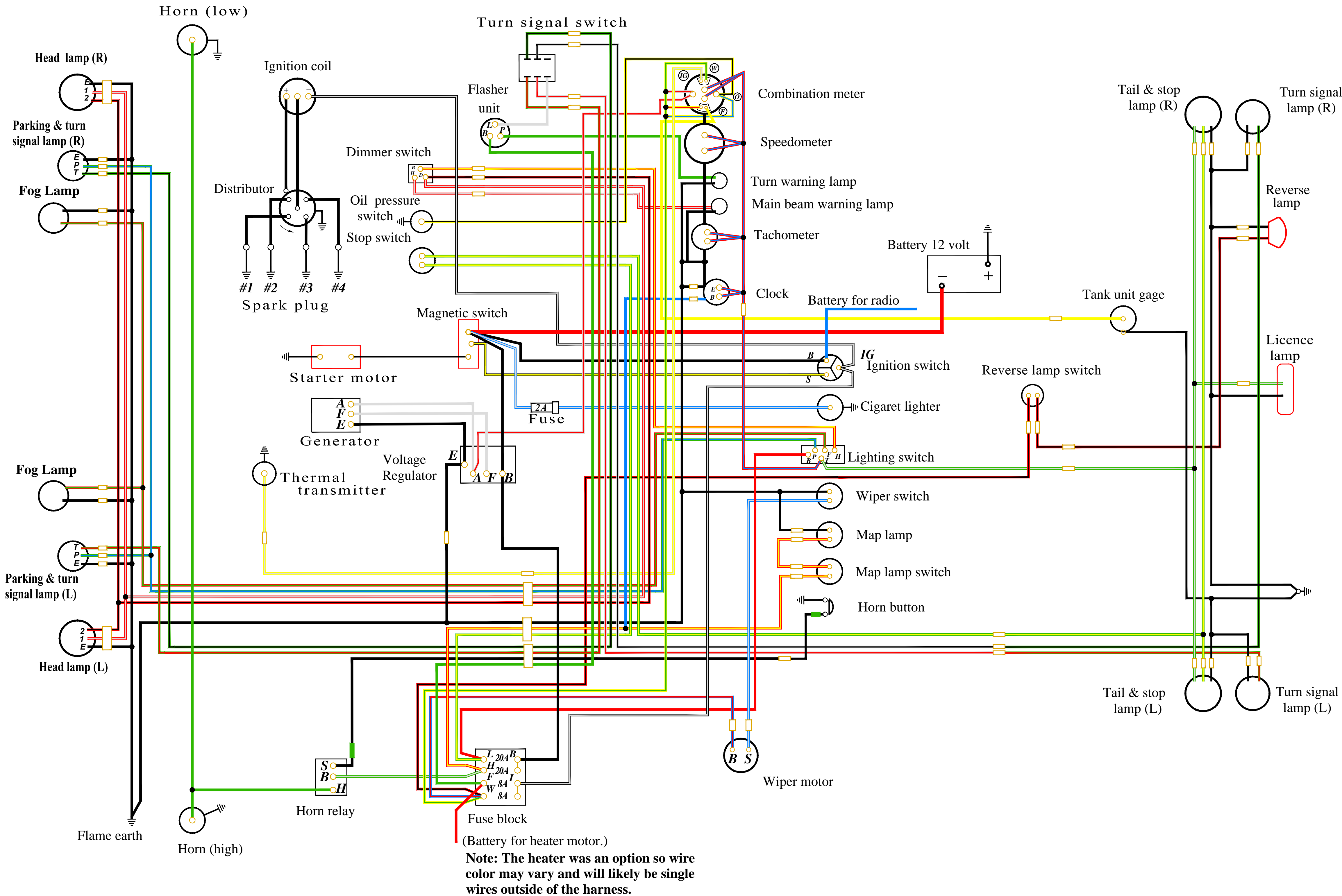
Schematic taken from red cover service manual for 3 seat, single carburetor model. Color version by Curtis Marsten 2015
