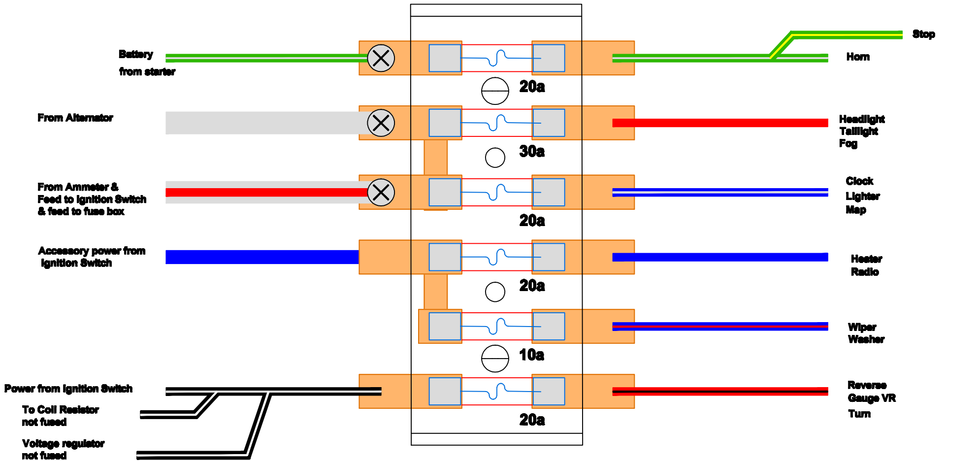
1968 Fuse Box
