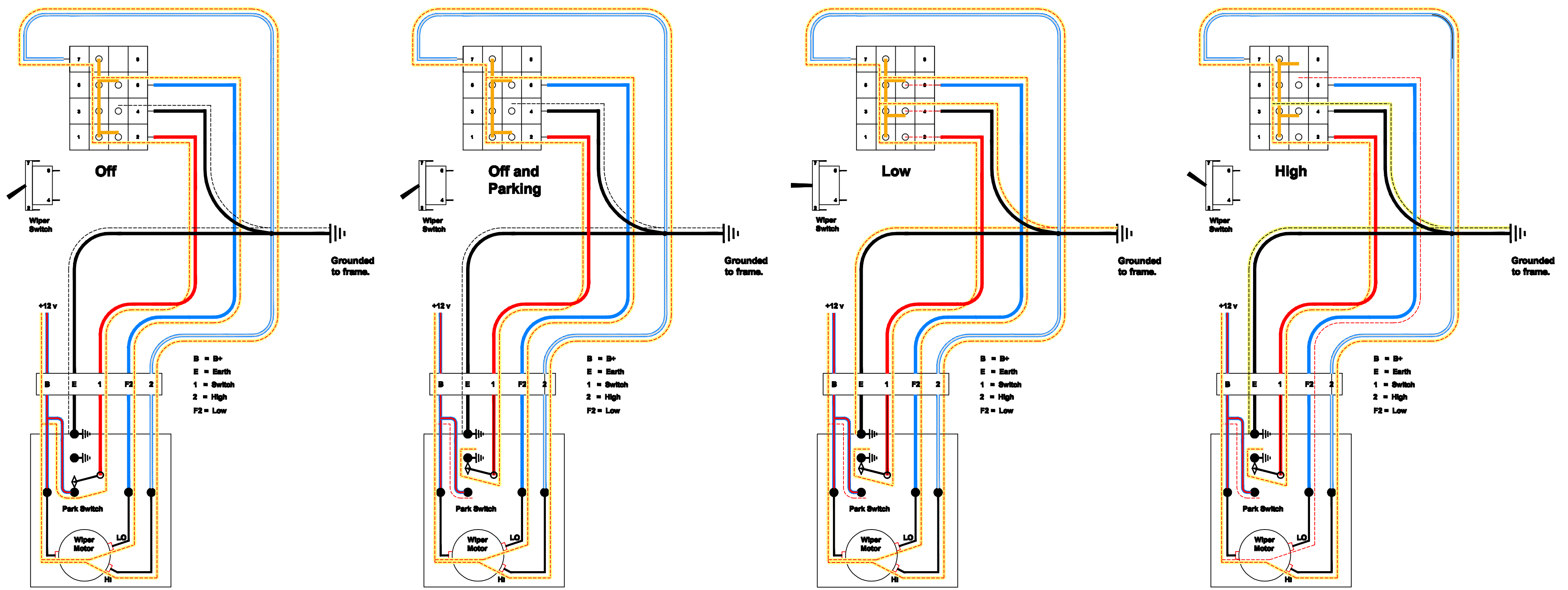
1966-67 Datsun SPL/SRL311 Wiper Circuits LHD Current Flow By Curtis Marsten ©2020
